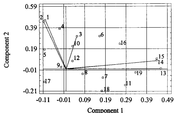
Figure 2. Plot of principal component weights. Key for numbers is that of Table 2.
