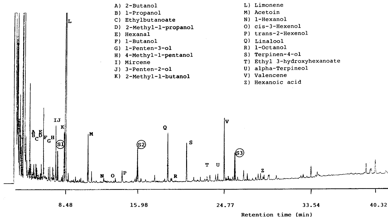
Figure 1. Gas chromatogram of aromatic components extracted from an orange juice.
